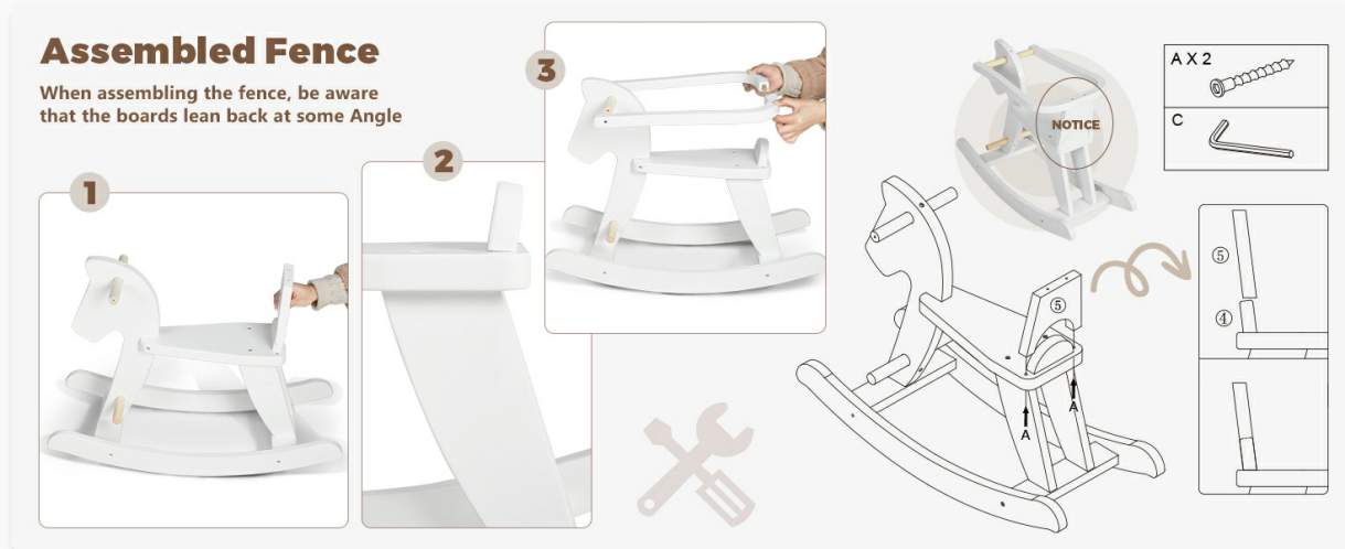
Image 2: Exploded view of the rocking horse components and included hardware.
