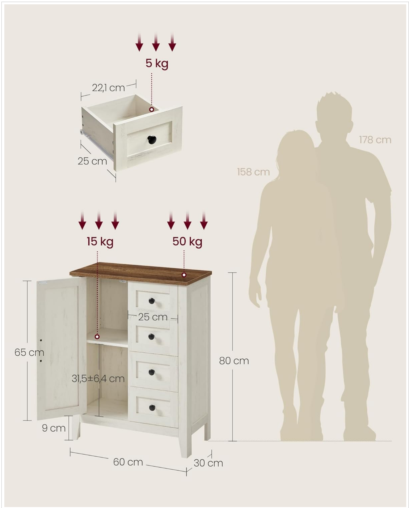
Image 8.1: Detailed dimensions and weight capacities for the cabinet and its components.
