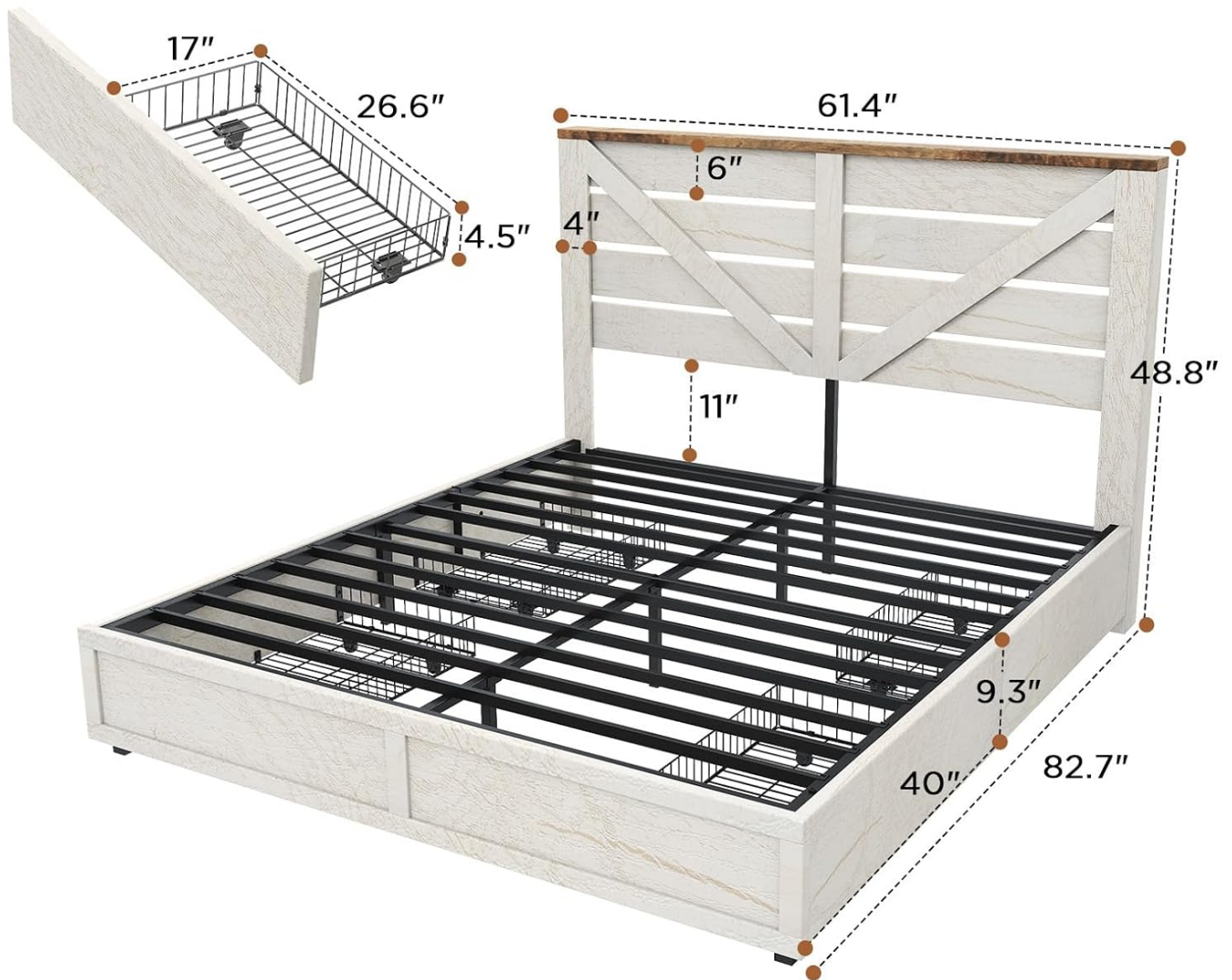
Figure 1: Bed Frame Dimensions and Capacity
