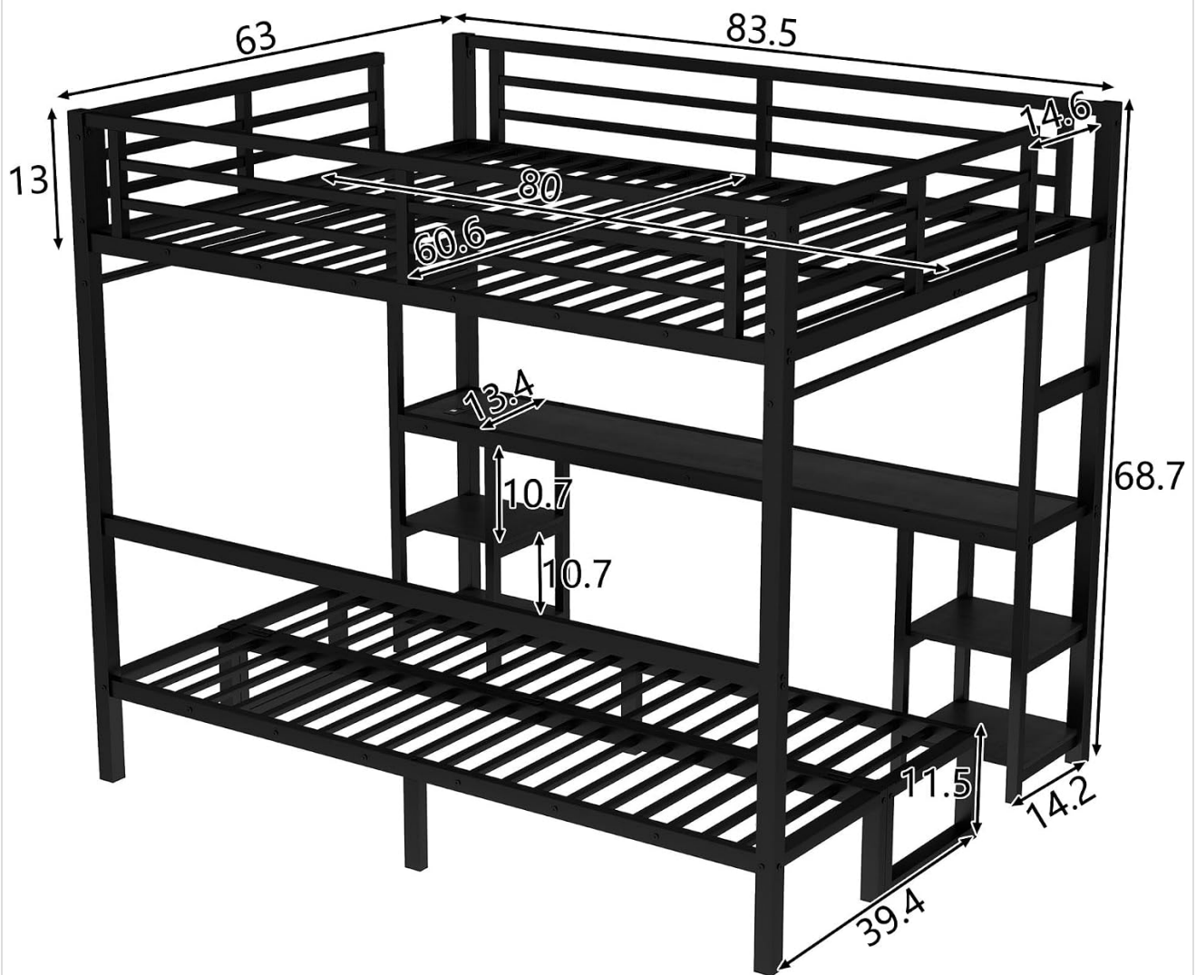
Figure 2: Product Dimensions.
