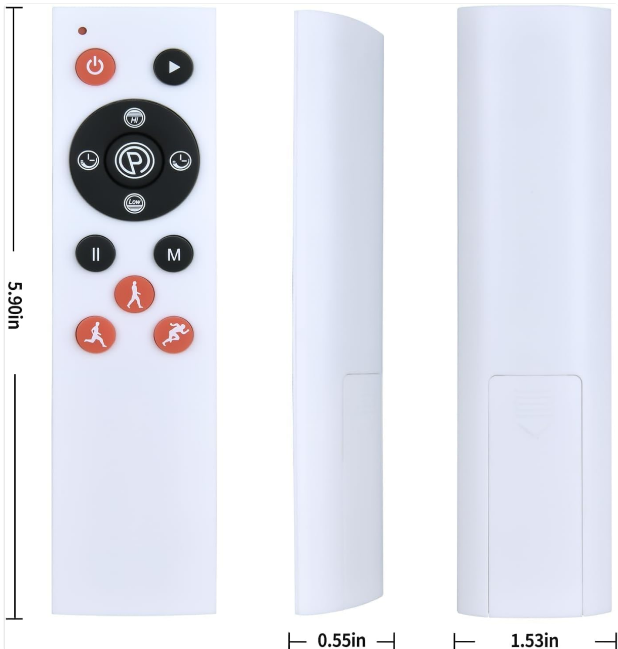
Figure 3: Remote control dimensions.
