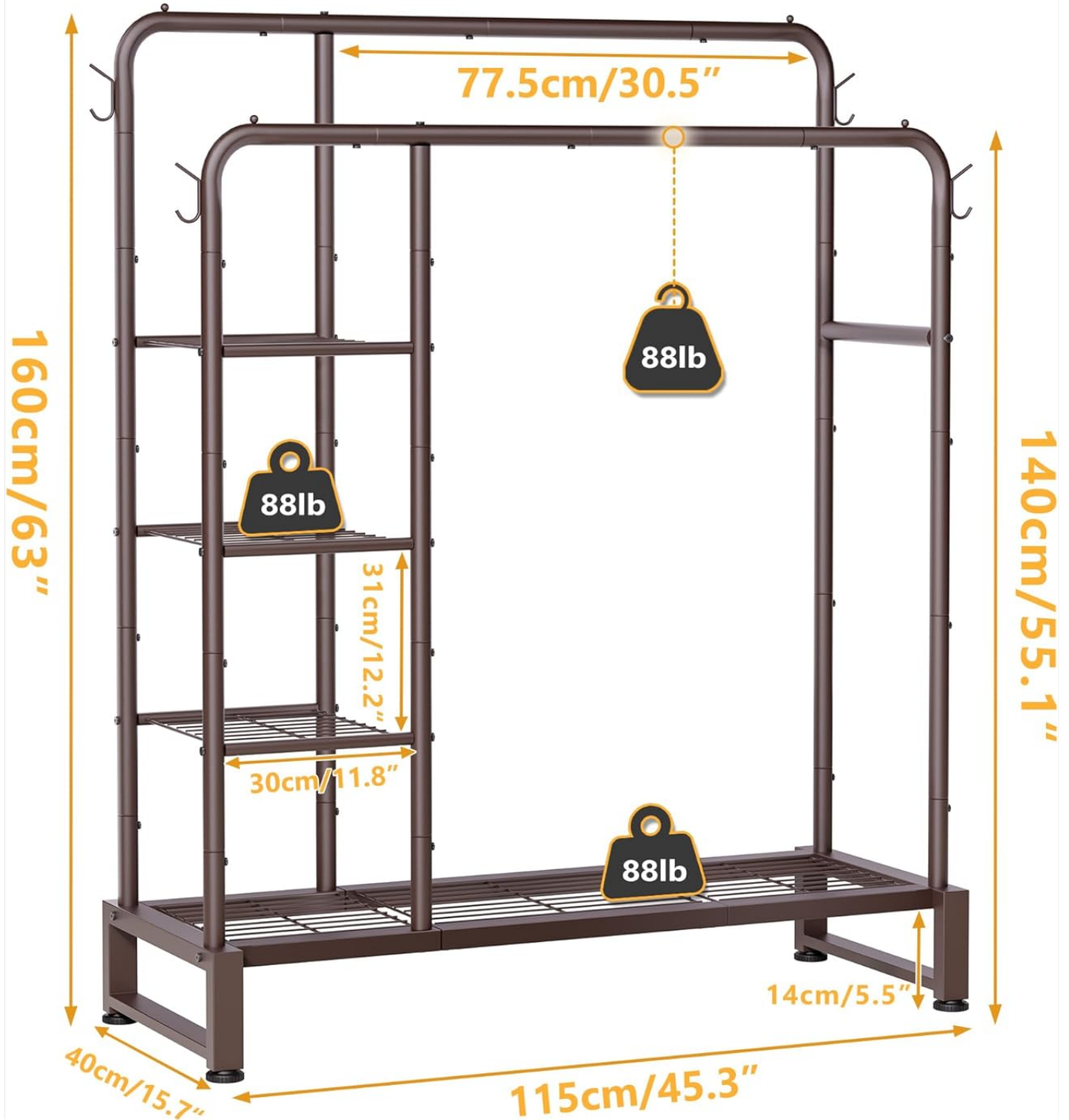
Image 8.1: Dimensional diagram of the clothes rack, including height, width, depth, and individual load capacities for rods and shelves.
