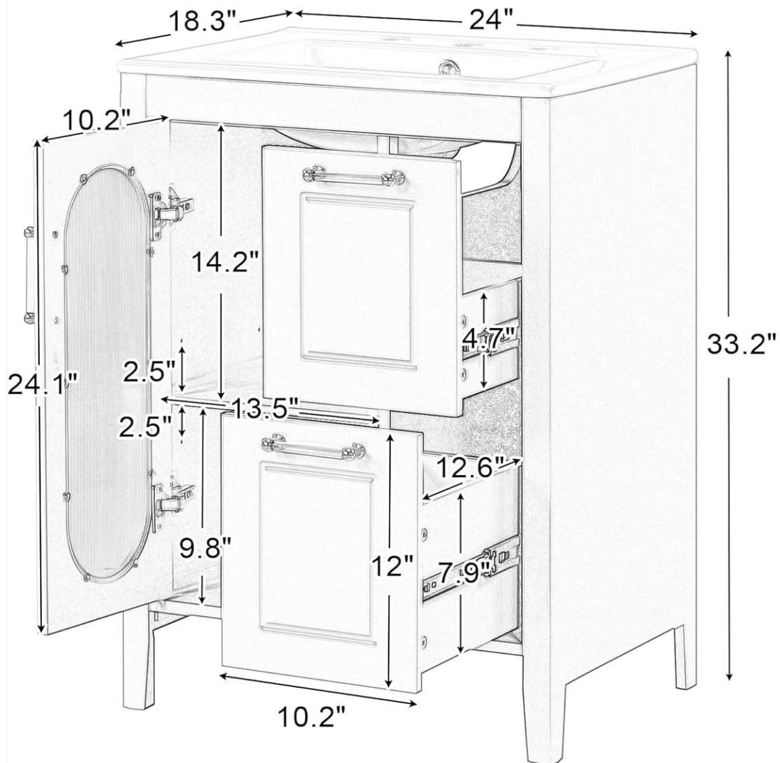
Image: Technical drawing illustrating the precise dimensions of the Linique 24-inch Bathroom Vanity in inches.
