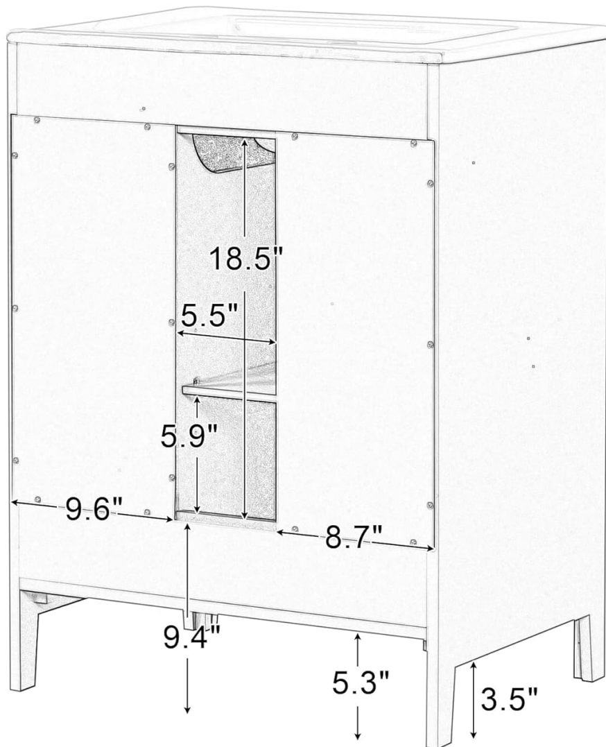
Image: Technical drawing showing the back view and specific dimensions of the Linique 24-inch Bathroom Vanity.
