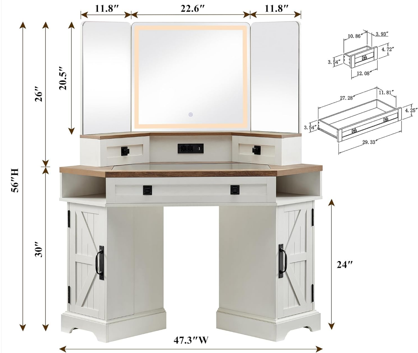
Image: Detailed product dimensions for the T4TREAM corner vanity desk.
