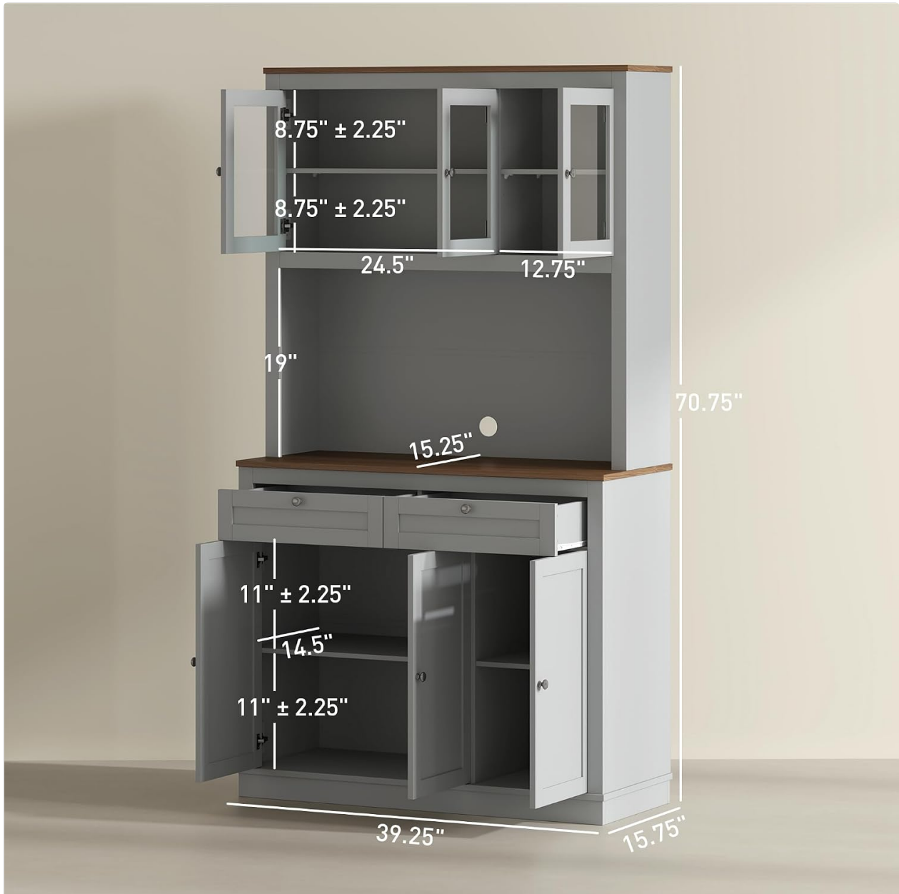
Image: Detailed dimensions of the HOMCOM Kitchen Pantry Cabinet.
