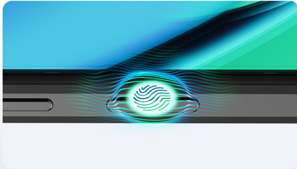
Side Fingerprint
