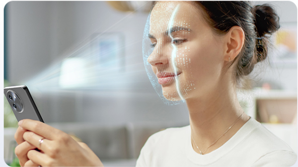
Face Recognition
