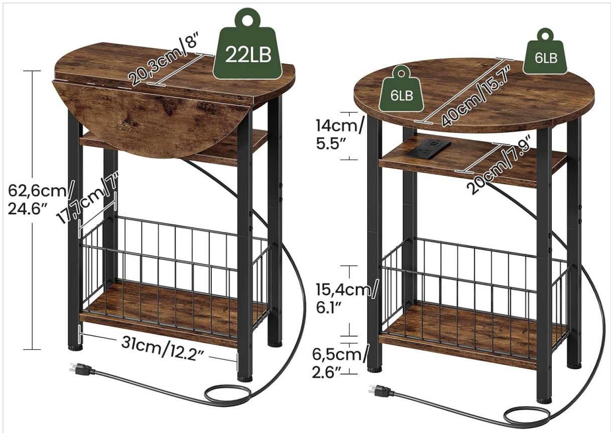
Image 8.1: Detailed dimensional diagram of the side table, illustrating measurements for both the folded and unfolded configurations, along with weight capacities.
