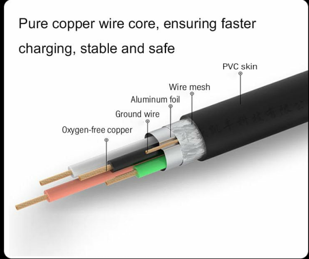
Figure 8.1: Internal and external components of the Xininyia magnetic charger.
