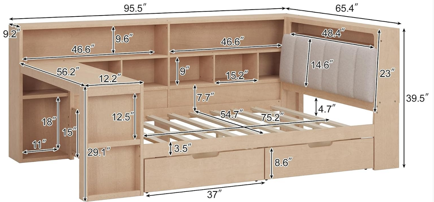
Figure 3.2: Detailed dimensions of the L-shaped daybed, including measurements for the bed frame, desk, and storage components.
