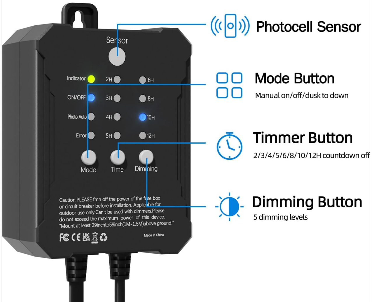
Image 4.1: Dusk to Dawn Sensor Controller interface.
