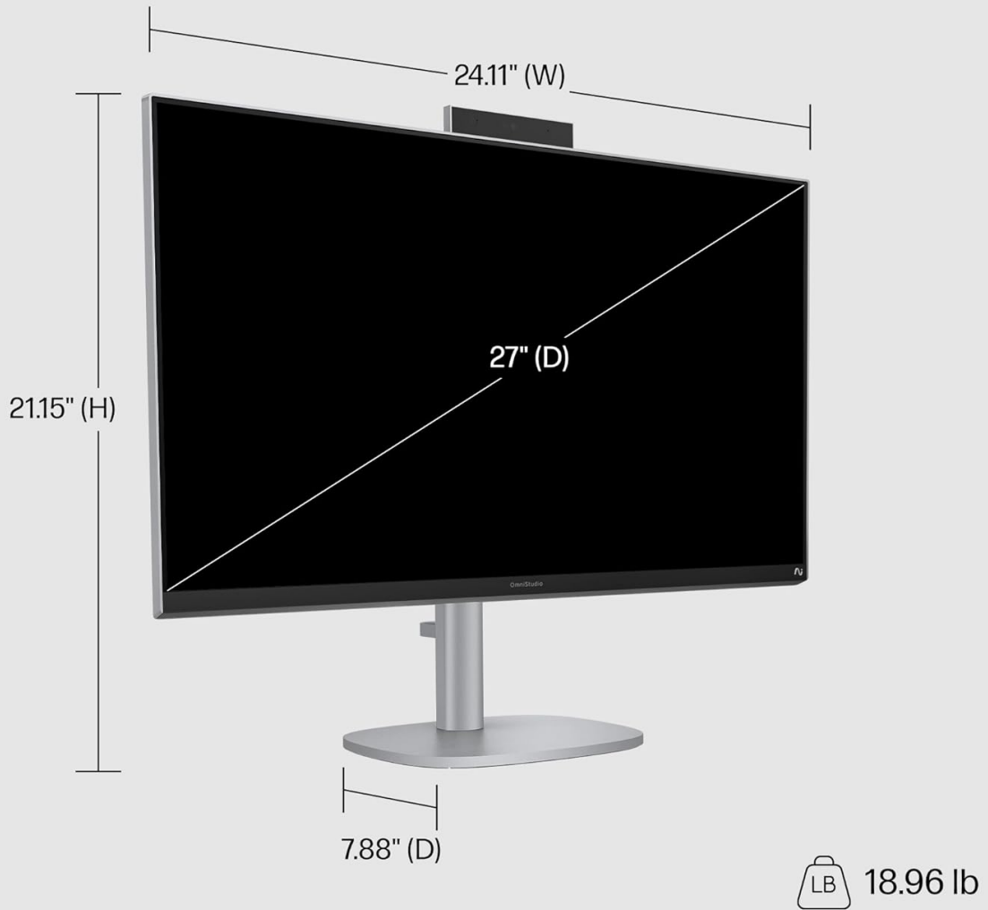
Image 7.1: Physical dimensions and weight of the HP OmniStudio X 27-inch All-in-One PC.
