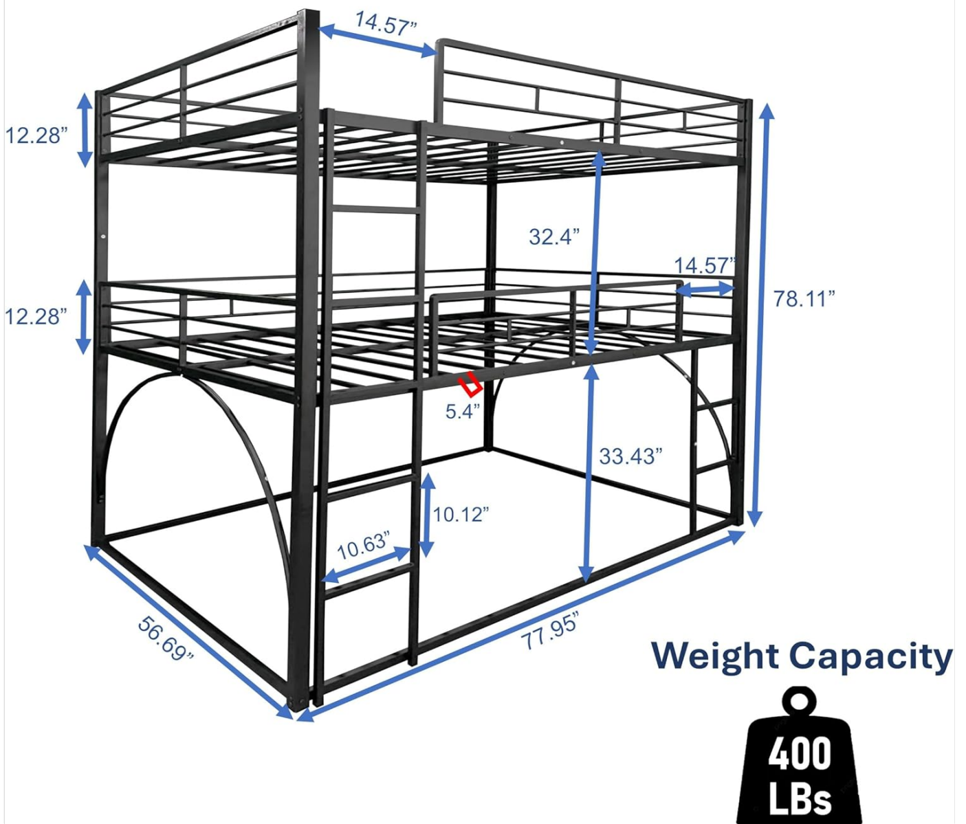
Figure 3: Product information diagram detailing dimensions (77.95"L x 56.69"W x 78.11"H) and weight capacity (400 lbs) for the UOCFYK Triple Bunk Bed. Please adhere to the 300 lbs weight limit per bed as stated in the safety information.
