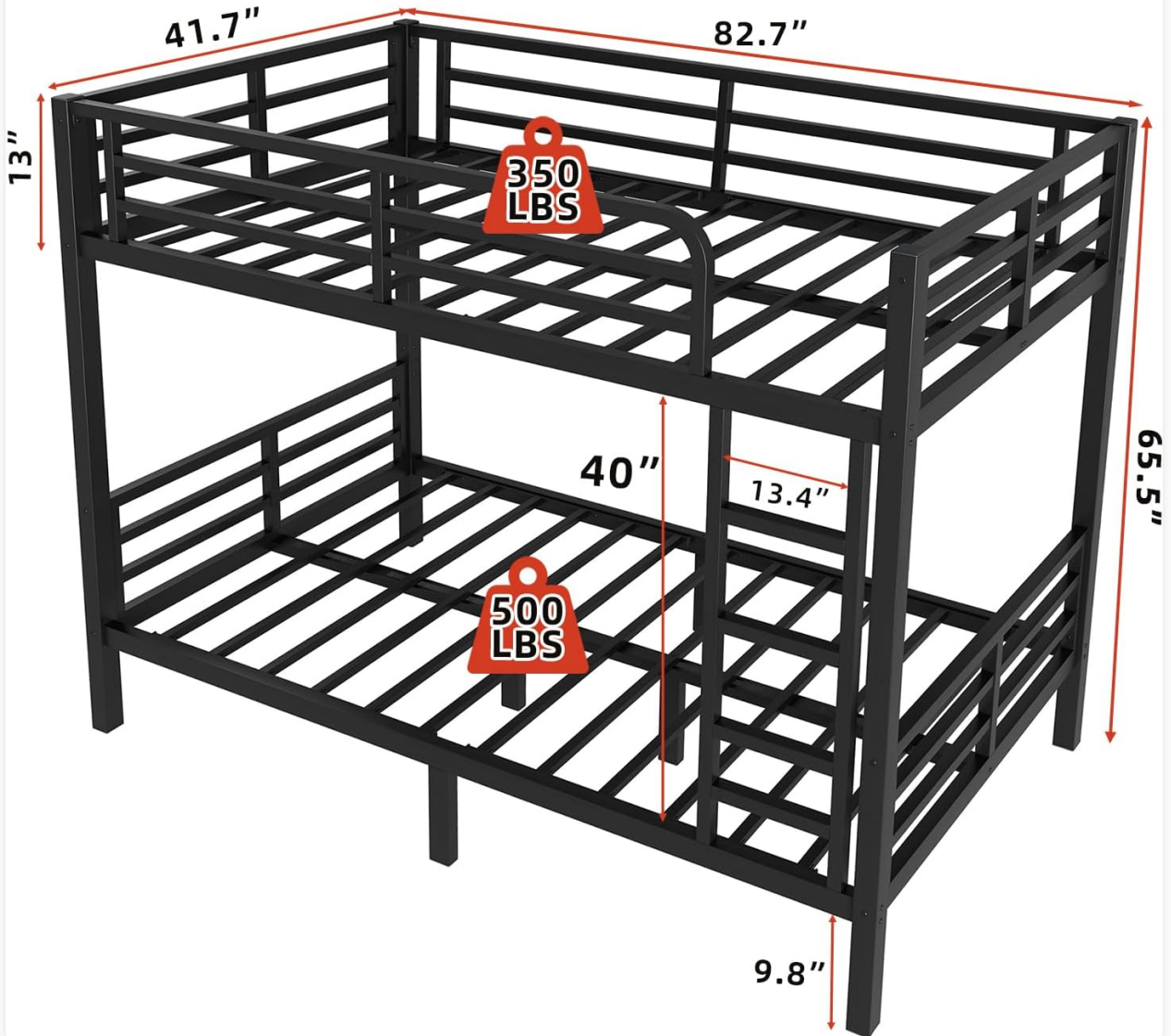
Image 4.1: Product dimensions for assembly reference.
