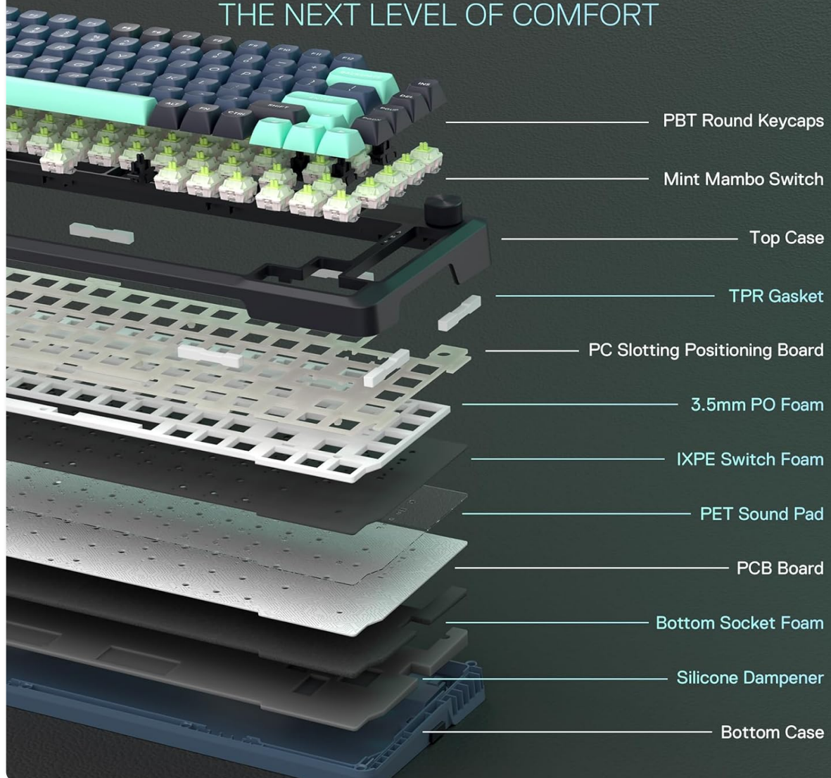
Image: Diagram illustrating the multi-layered gasket design for enhanced typing comfort and reduced noise.
