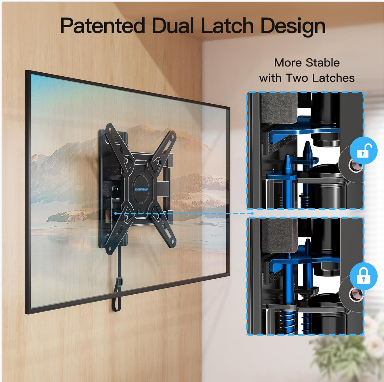
Figure 5: Close-up of the patented dual latch design, showing locked and unlocked positions.
