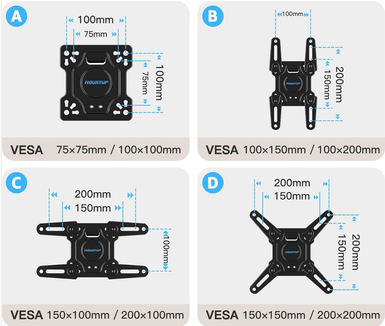
Figure 4: Detailed VESA pattern compatibility chart.
