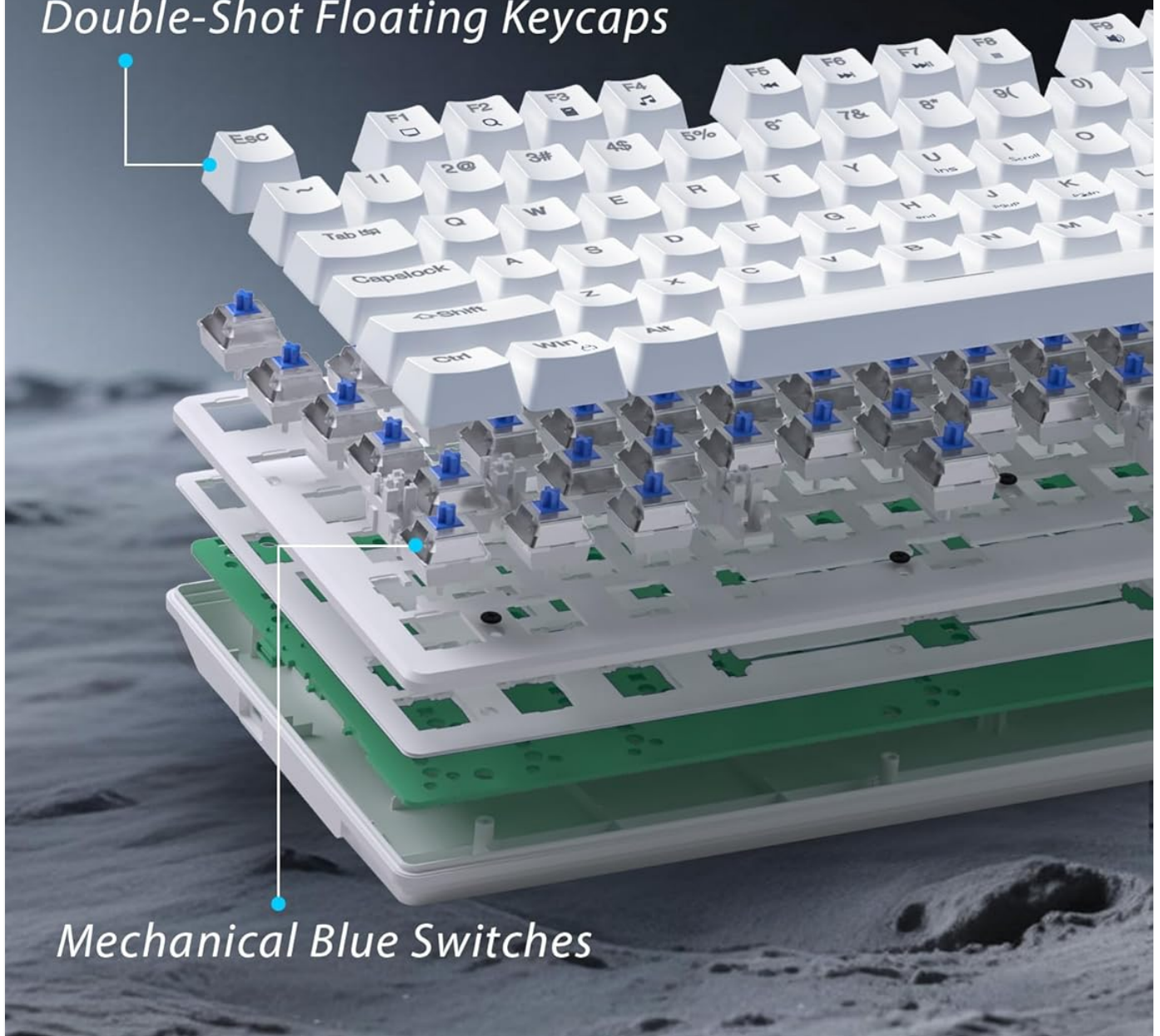
Image 3.1: Exploded view illustrating the internal structure of the mechanical keyboard, highlighting the double-shot floating keycaps and mechanical blue switches.
