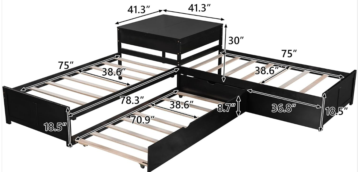
Image 6.1: The L-shaped platform bed with the trundle bed fully extended, demonstrating its additional sleeping capacity.
