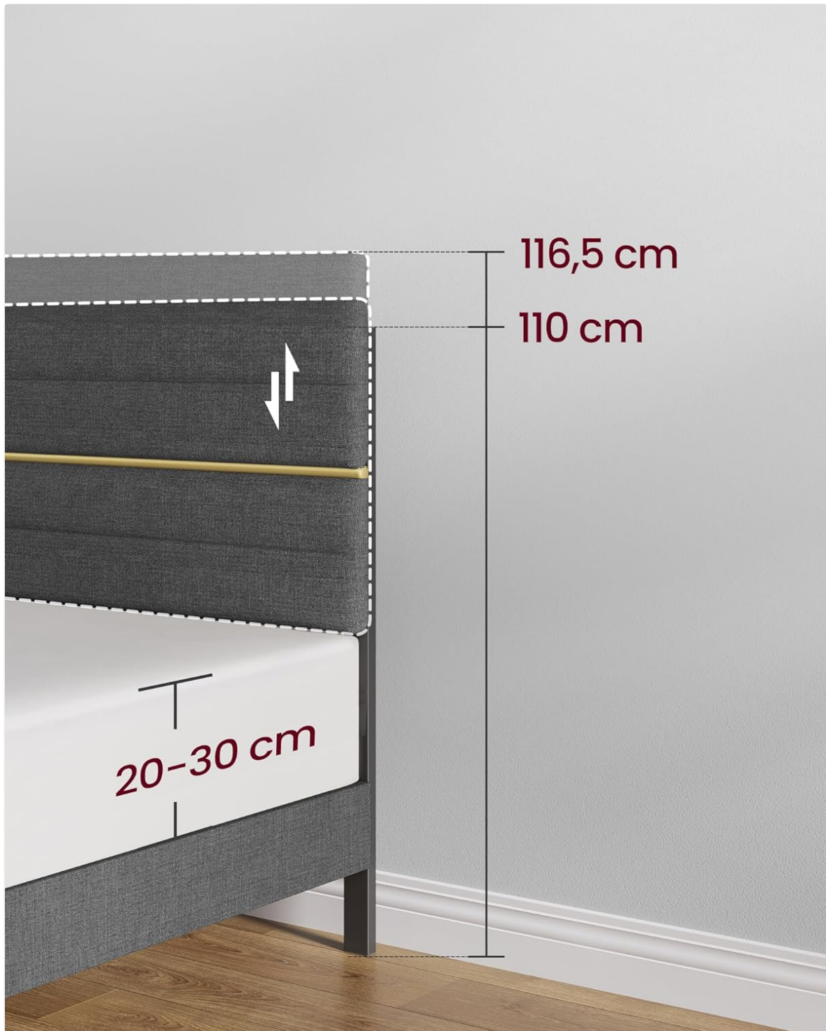
Figure 3: Adjustable headboard height. The headboard can be set at 110 cm or 116.5 cm to accommodate mattresses with a thickness between 20 cm and 30 cm.
