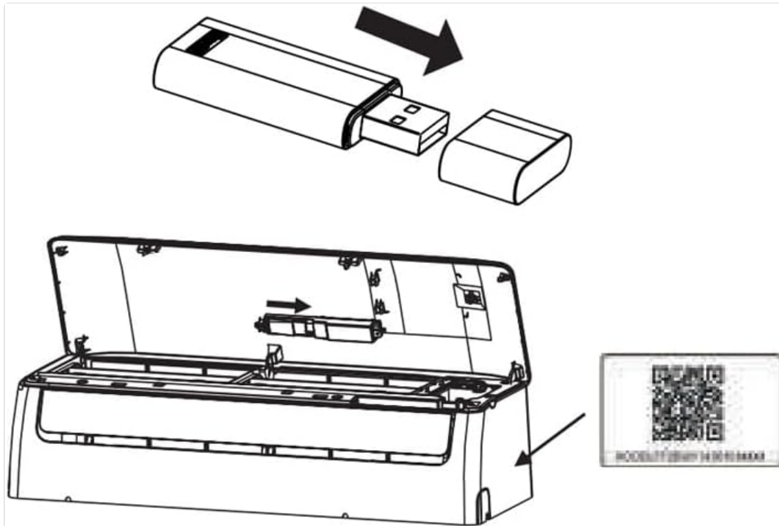
Figure 4: Diagram illustrating the process of inserting the USB WiFi module into the dedicated port of an air conditioning unit. A QR code is also shown, likely for app pairing.
