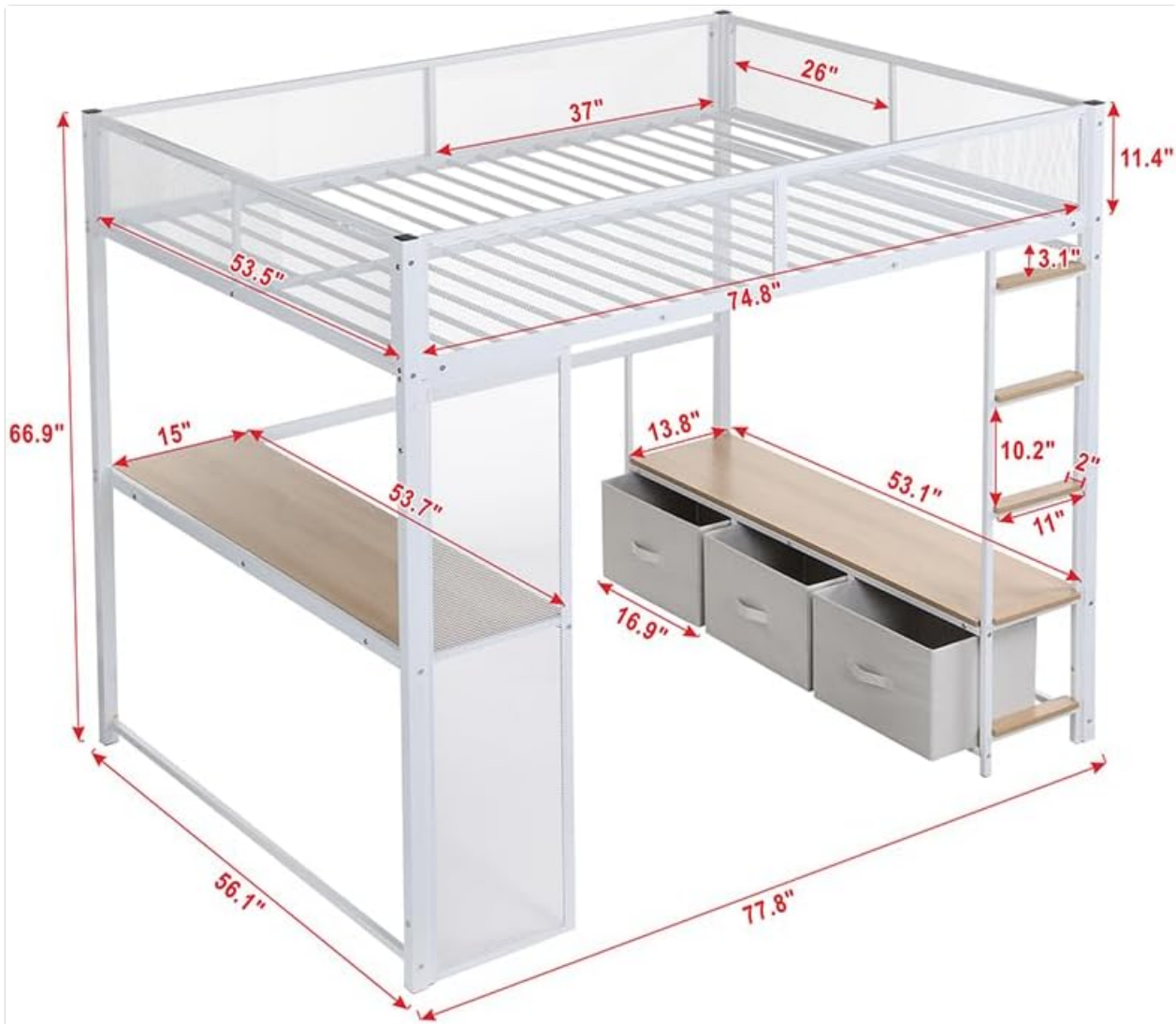
Image: Detailed dimensions diagram of the SOFTSEA Full Gaming Loft Bed.
