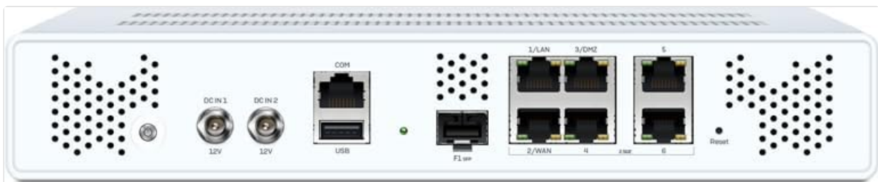
Image: Rear view of the Sophos XGS 108 appliance, displaying power inputs, a console port, USB ports, multiple 2.5 GE copper ports, and an SFP fiber port.
