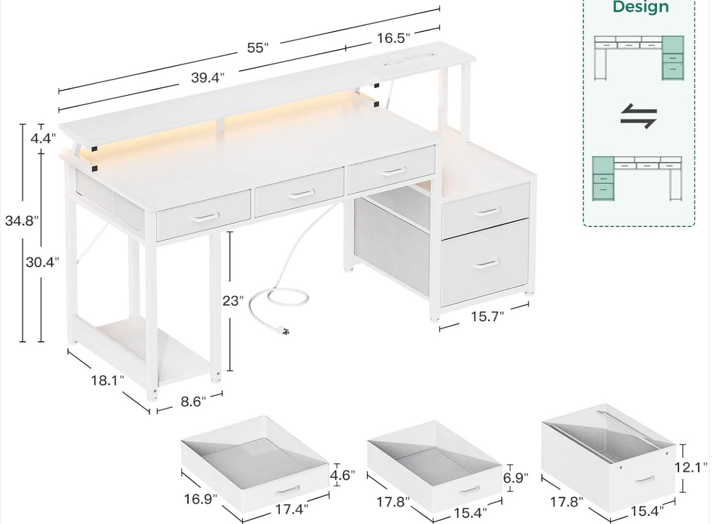
Figure 3.1: Product dimensions, useful for planning your space and during assembly.
