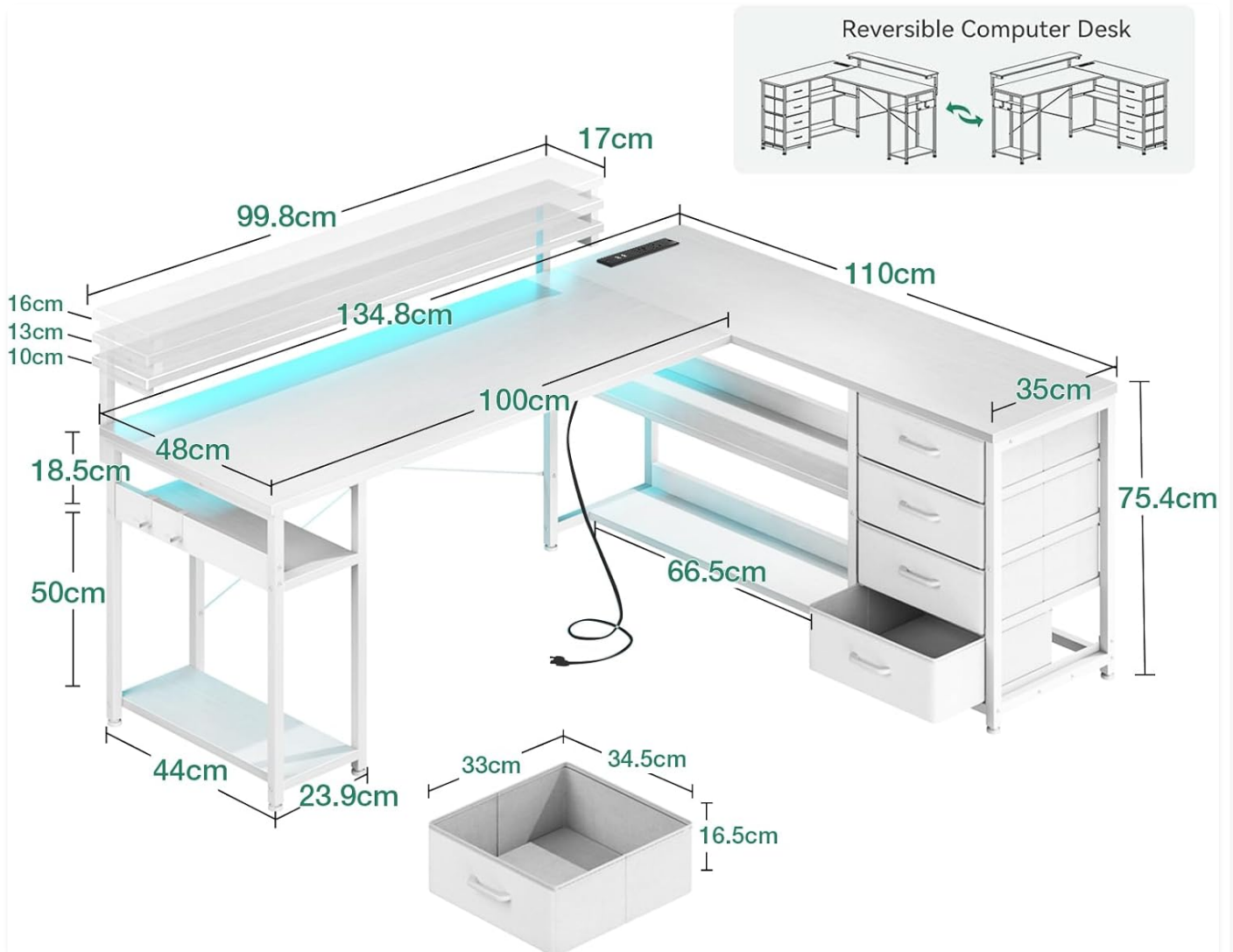
Figure 2: Dimensional diagram and illustration of the reversible L-shaped design, allowing for flexible setup.
