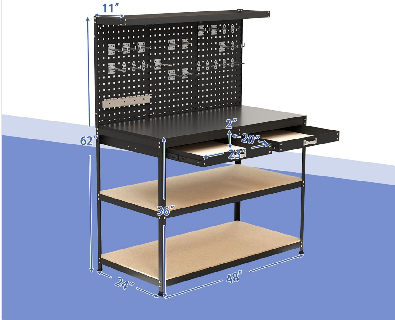
Image: Overview of Goplus Workbench product dimensions, showing height, width, and depth of various components.
