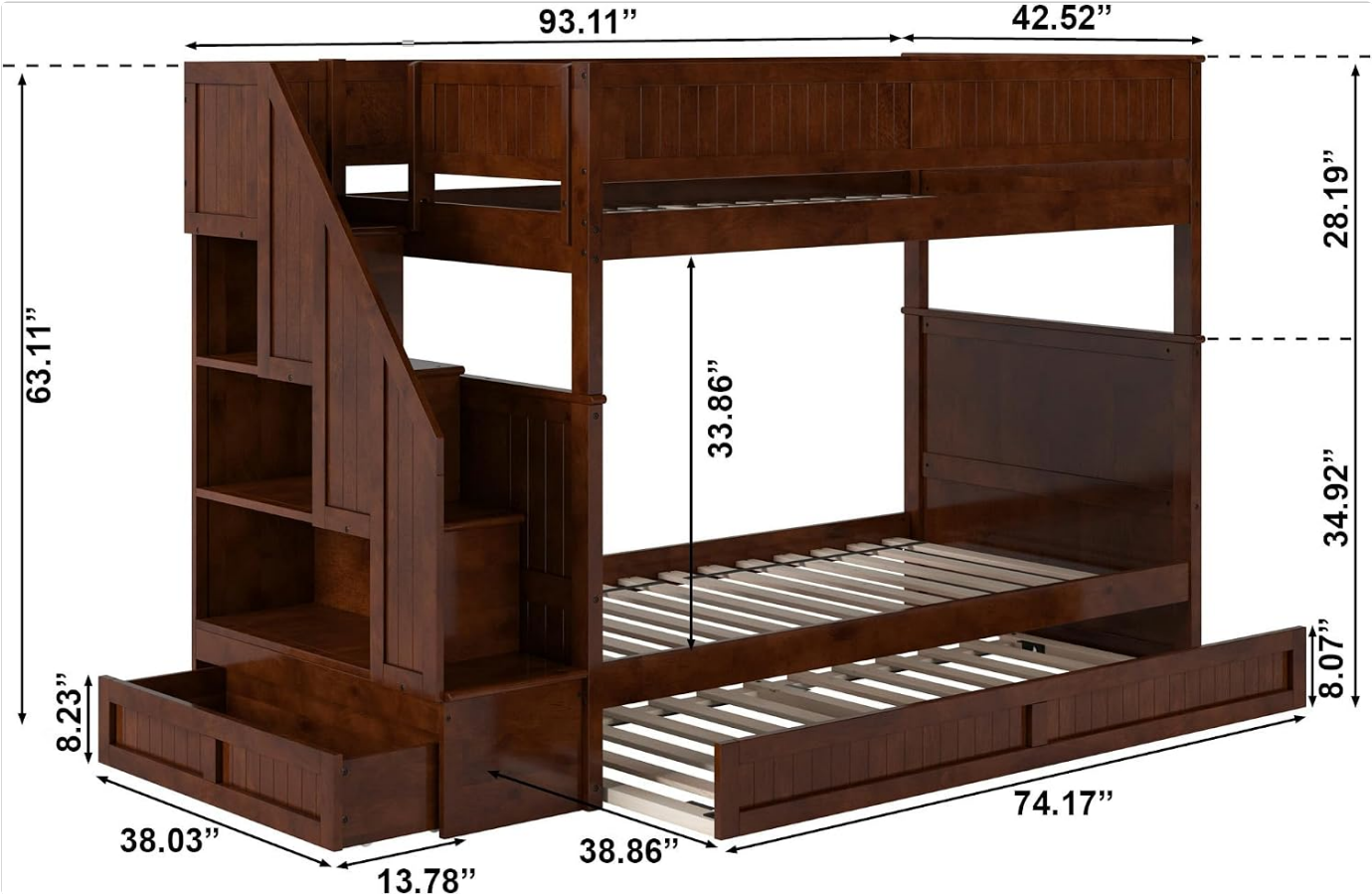
Image: Technical drawing illustrating the full dimensions of the AFI Dover Twin Over Twin Staircase Bunk Bed, including length, width, height, and individual component measurements.
