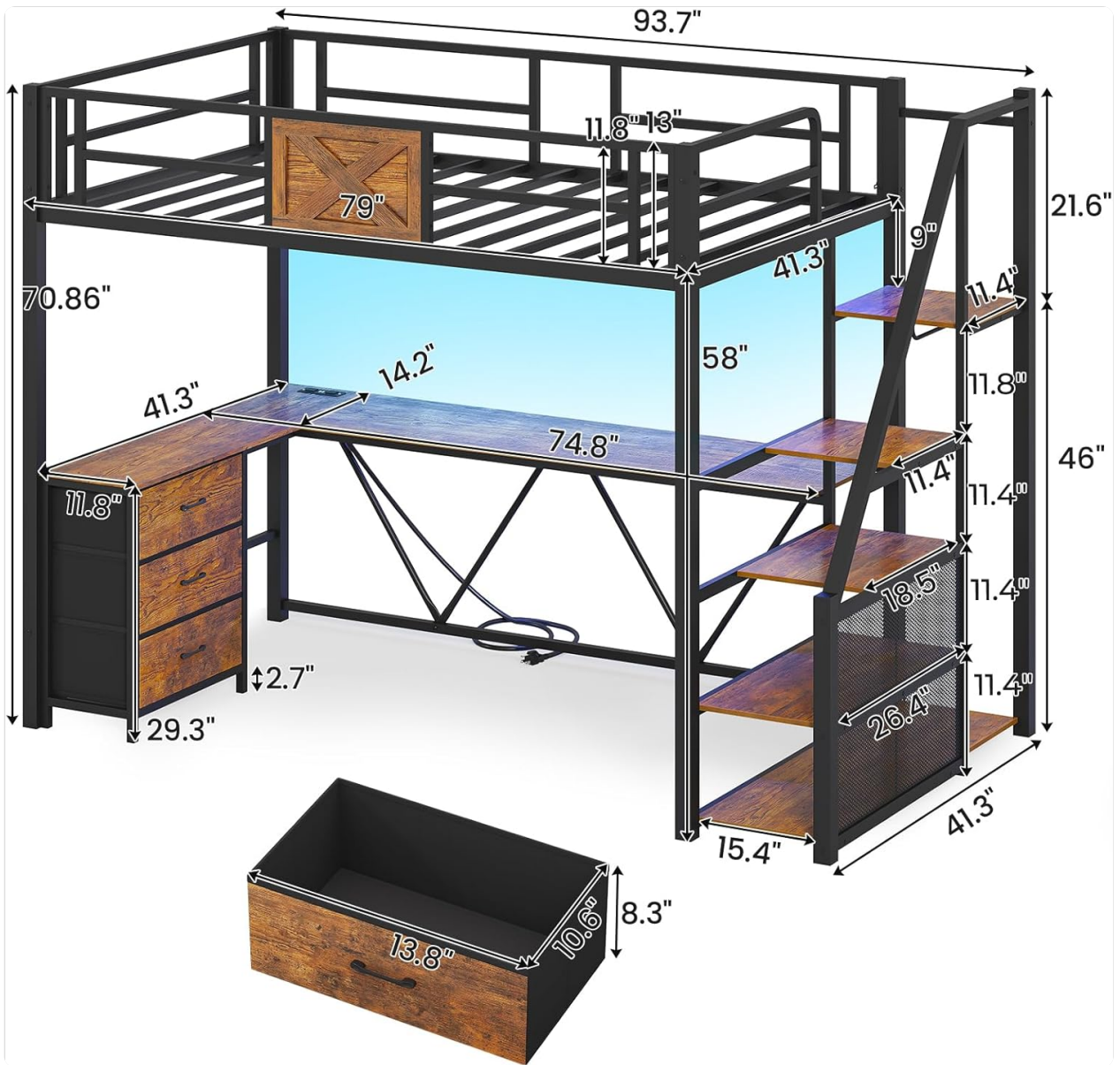
Figure 9: Product dimensions and key measurements.
