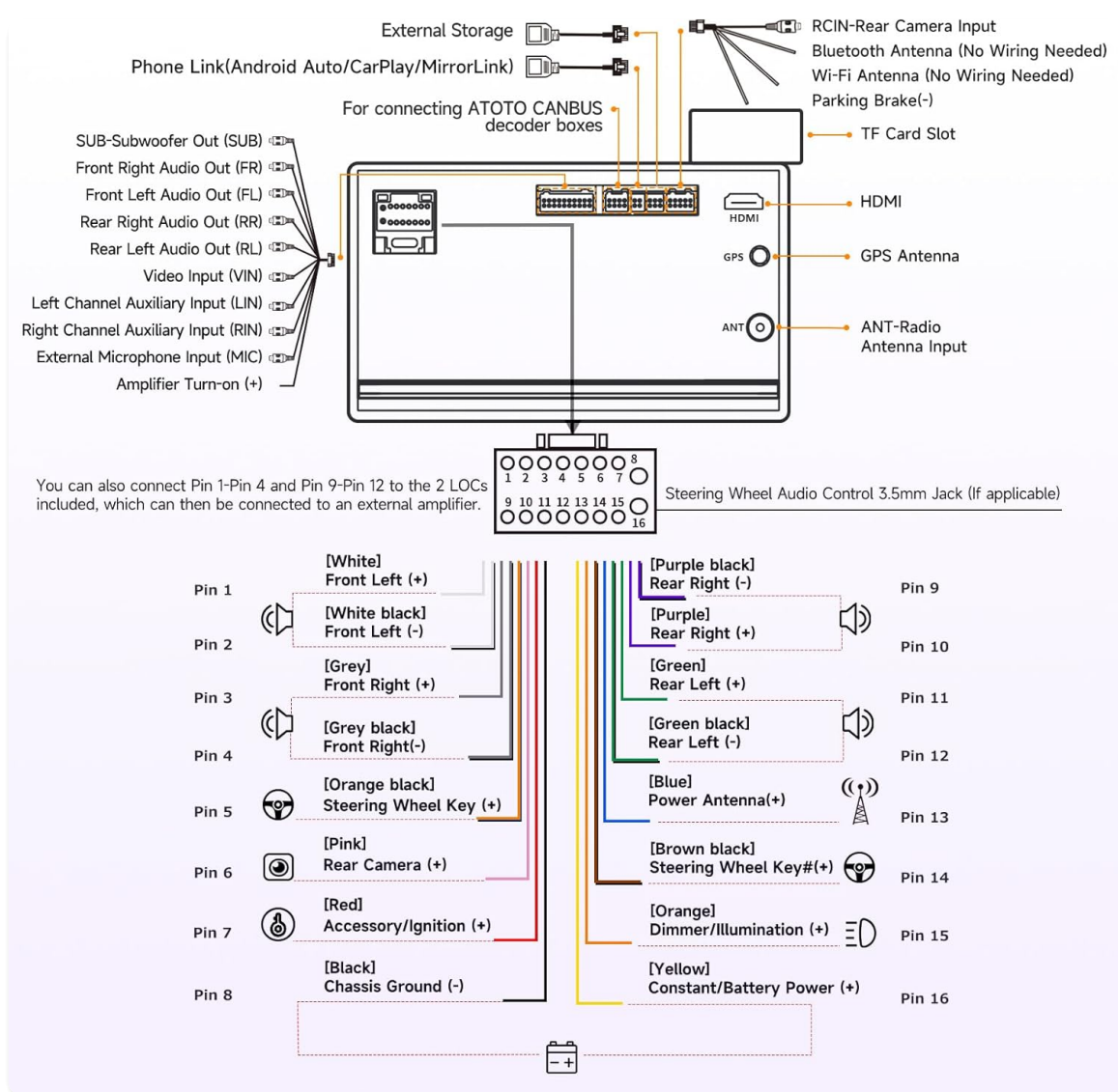
Image 3.1: Detailed wiring connections for the ATOTO A5L head unit.
