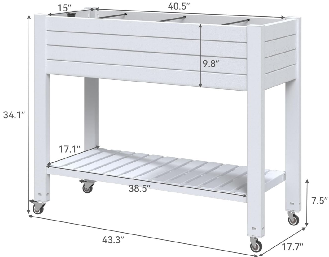
Image: A technical diagram detailing the product dimensions (length, width, height, and internal measurements) and indicating a 21-gallon capacity with a weight capacity of 230 lbs.
