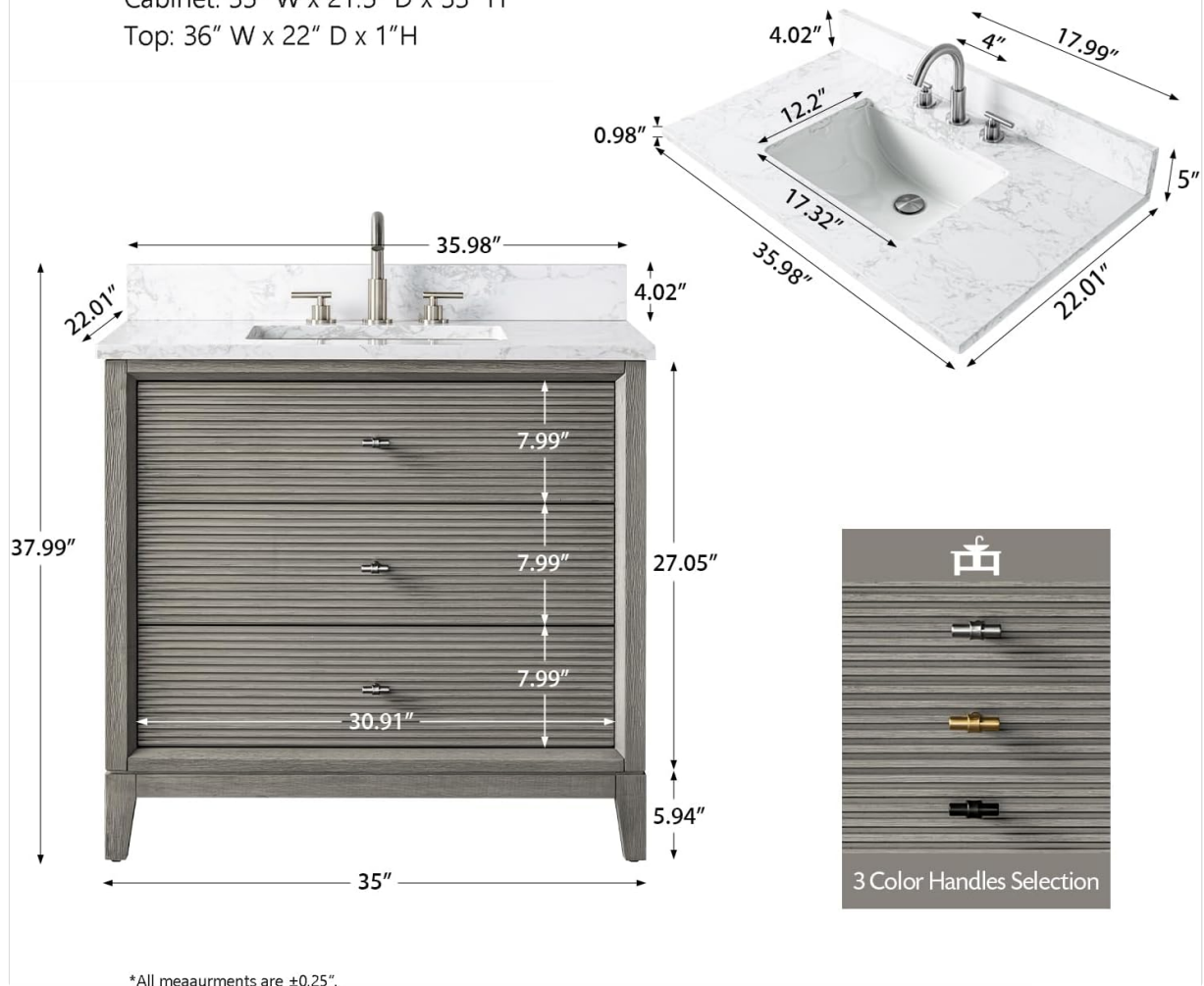
Figure 2: Overall Dimensions (36" W x 22" D x 38" H)
