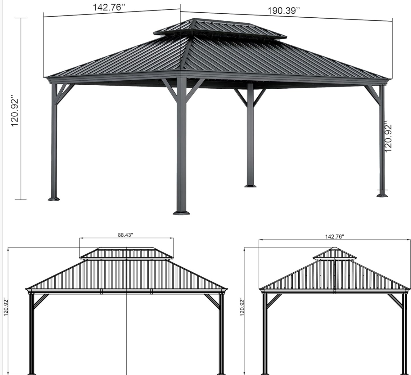
Image 8.1: Dimensional overview of the gazebo.
