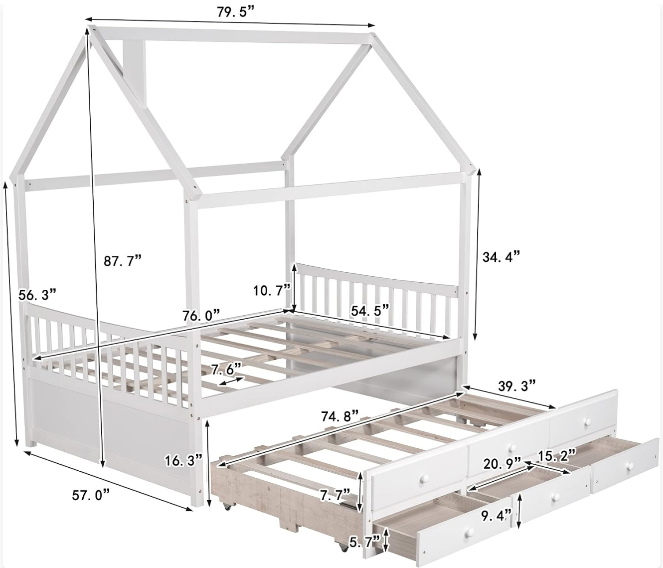
Image 8.1: Detailed dimensions of the bed frame.
