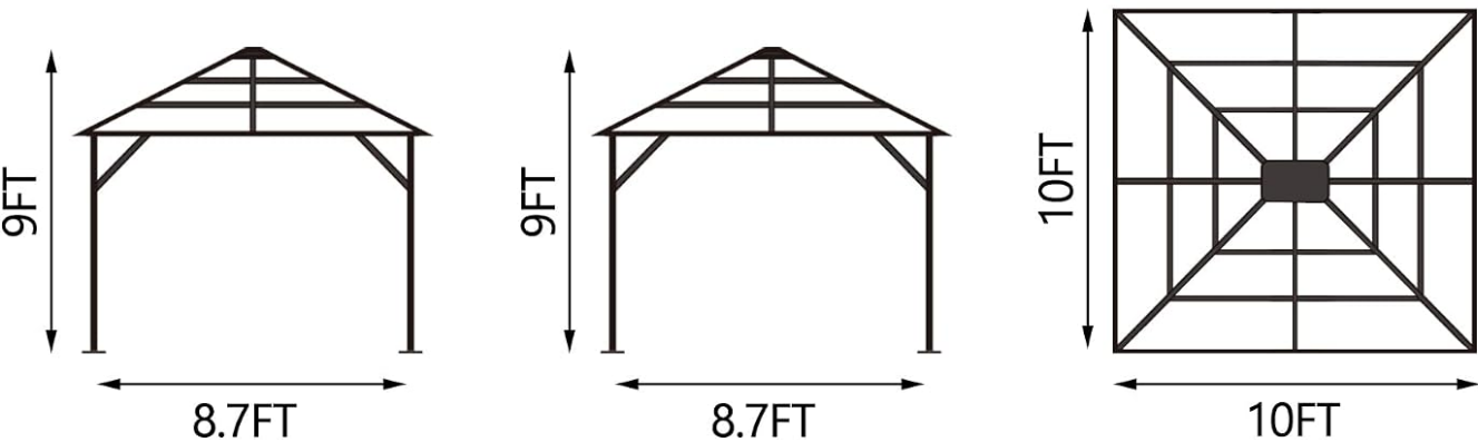
Image: A technical drawing illustrating the overall dimensions of the 10x10FT gazebo, including roof and base measurements.
