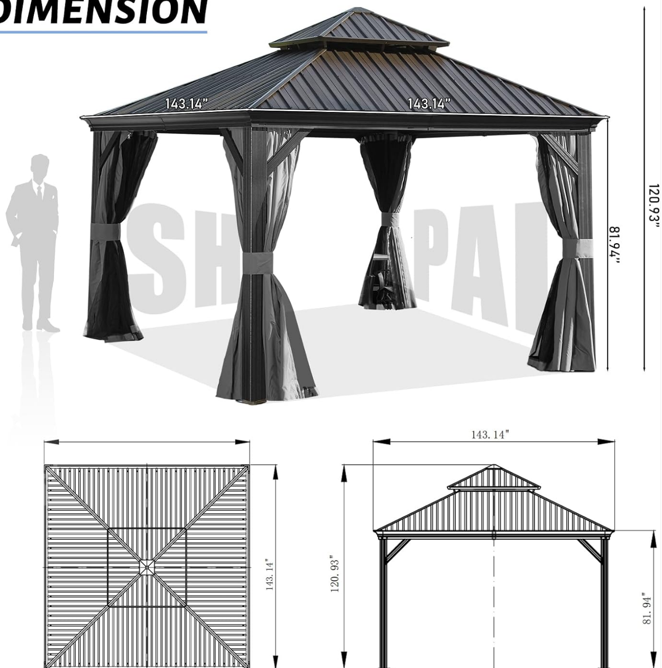
Image 4: A detailed diagram illustrating the overall dimensions of the SHPAI Gazebo, including length, width, and height measurements, crucial for planning installation space.
