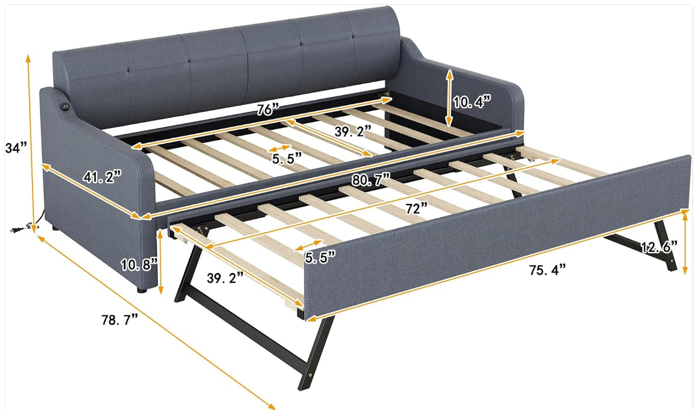
Image: Diagram showing the overall dimensions and key measurements of the daybed and its pull-out trundle.
