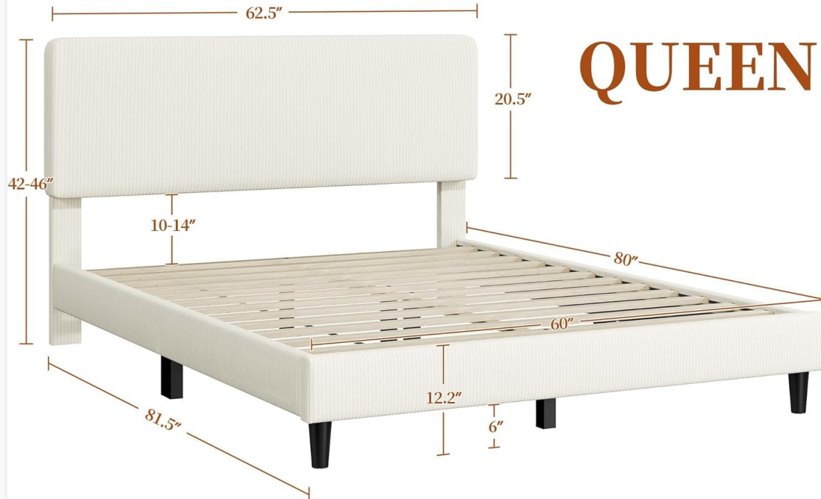
Figure 7: Key dimensions and weight capacity of the bed frame.
