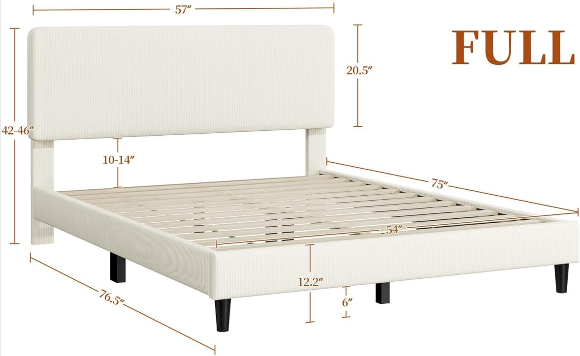
Image 8.1: Detailed dimensions of the Yaheetech Full Size Bed Frame.
