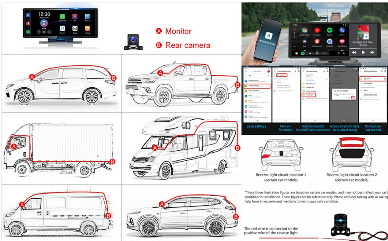
Figure 3.2: Rear camera installation and wiring diagrams for various vehicle types.
