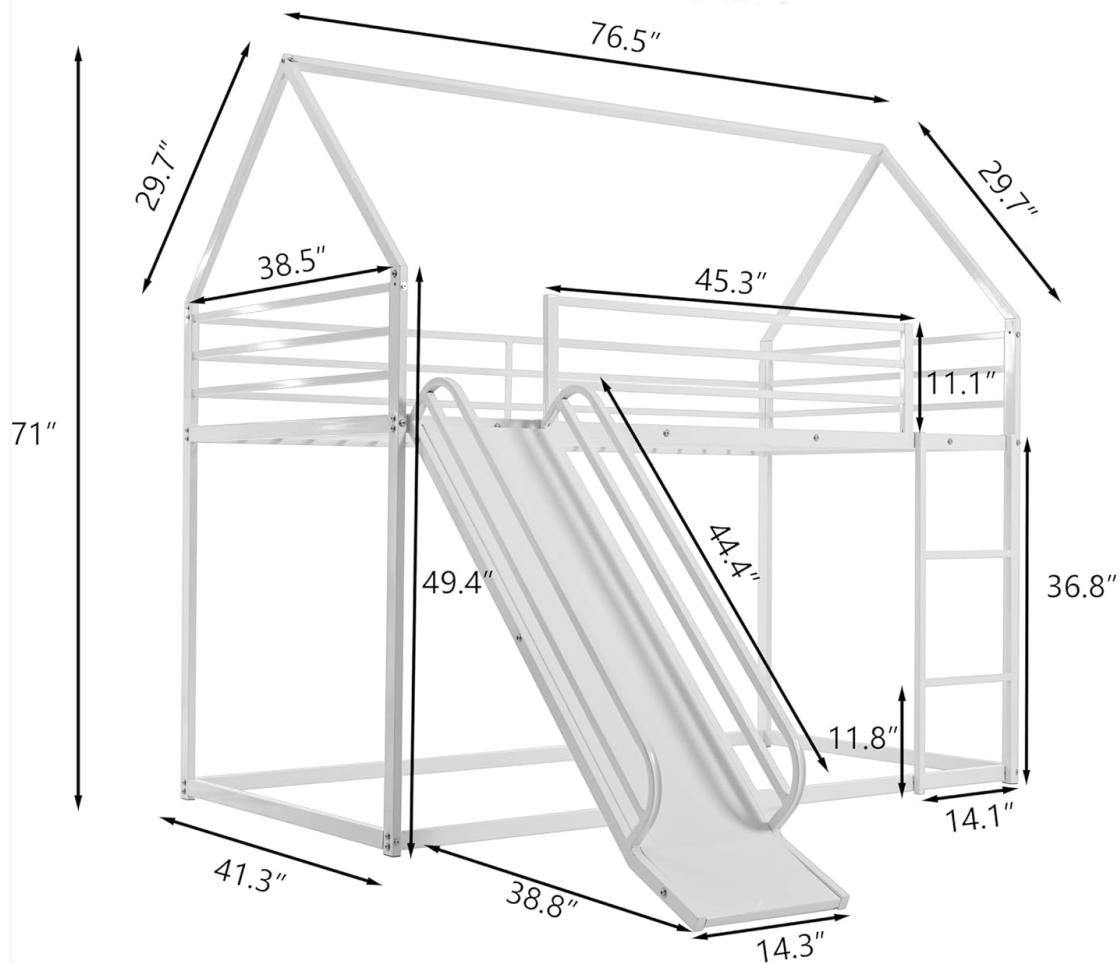
Image 1.1: Assembled EMKK Metal Bunk Bed with Slide in a bedroom setting.
