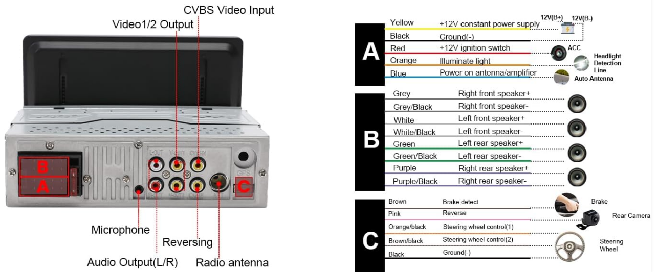
Image 3.1: Wiring diagram and dimensions of the car radio unit.
