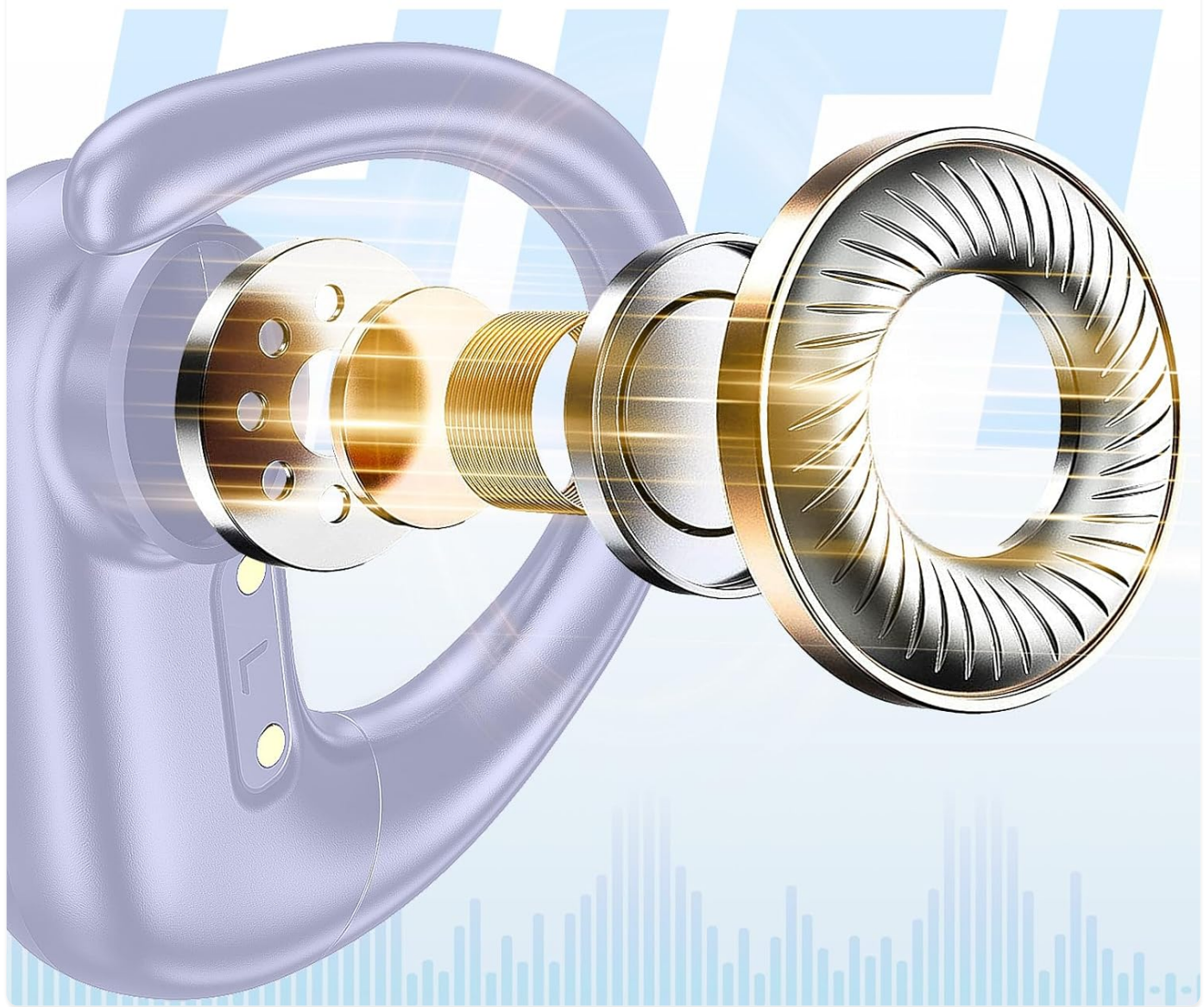
Image: An exploded view of the earbud's internal structure, emphasizing the 10mm Graphene Diaphragm for Hi-Fi stereo sound.
