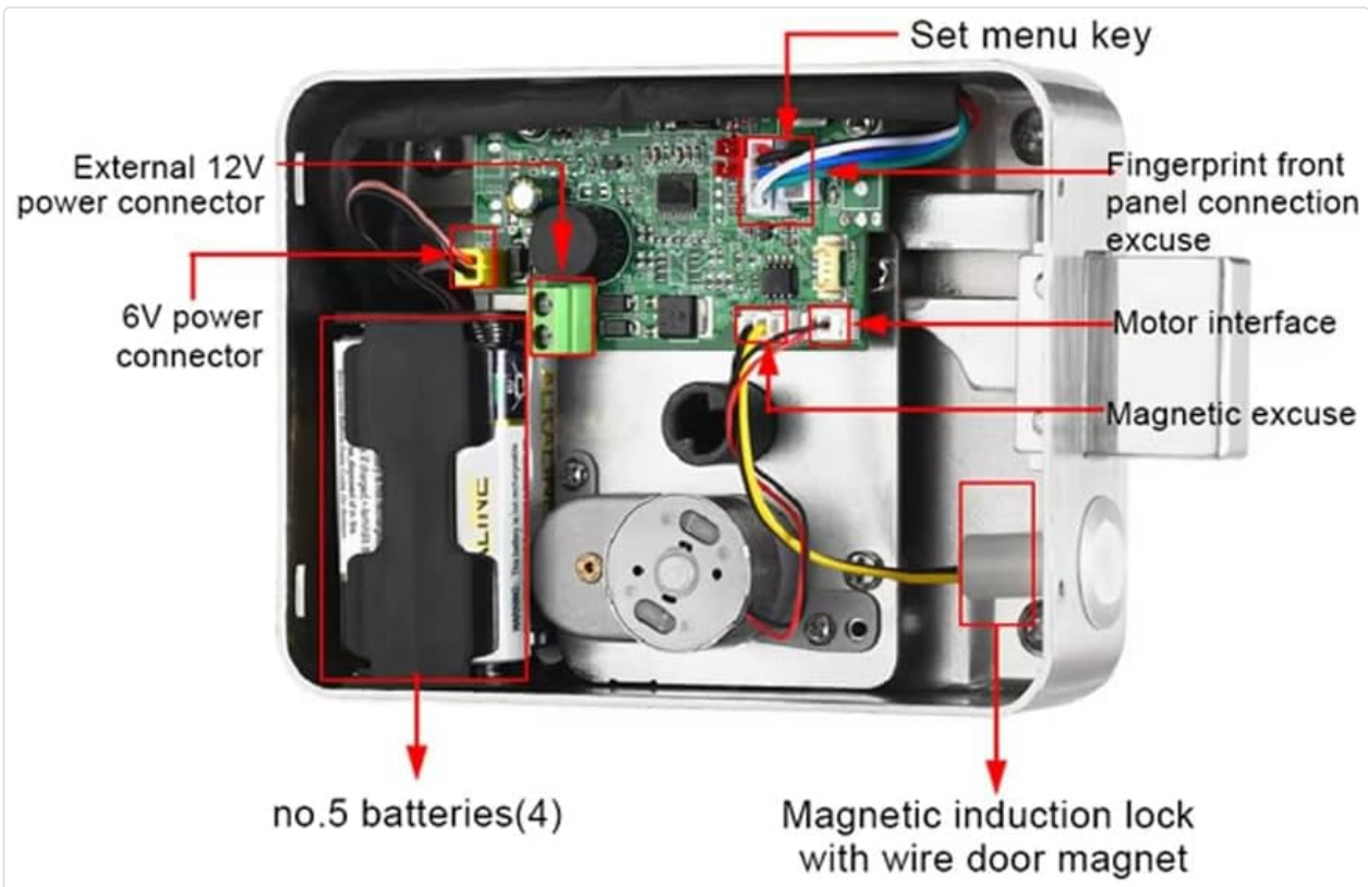
Figure 3.1: Internal components of the Razuvious M3 Smart Door Lock, including battery compartment and wiring points.
