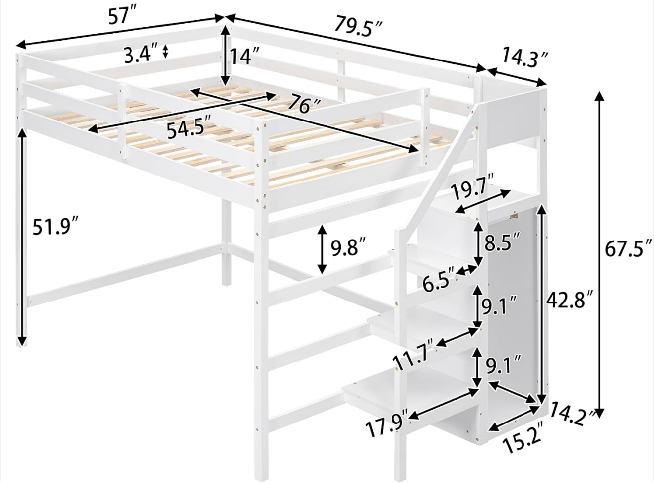
Figure 5: Detailed dimensions of the loft bed in inches.
