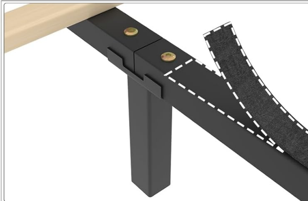
Figure 2: Assembly and Construction Details. This image illustrates the easy assembly process, the composite solid construction for durability, and the EVA mute bars for noise-free operation.
