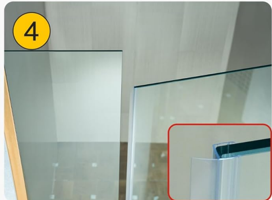
PVC strip on the outside of the hinged door
