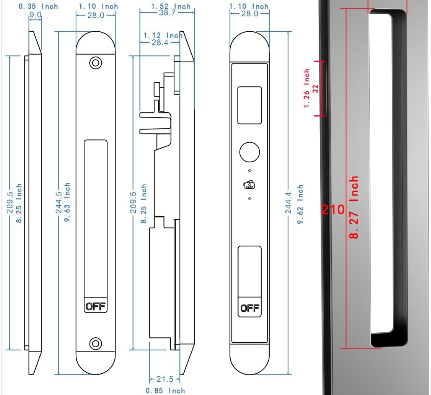
Figure 6.2: Detailed dimensions for installation.
