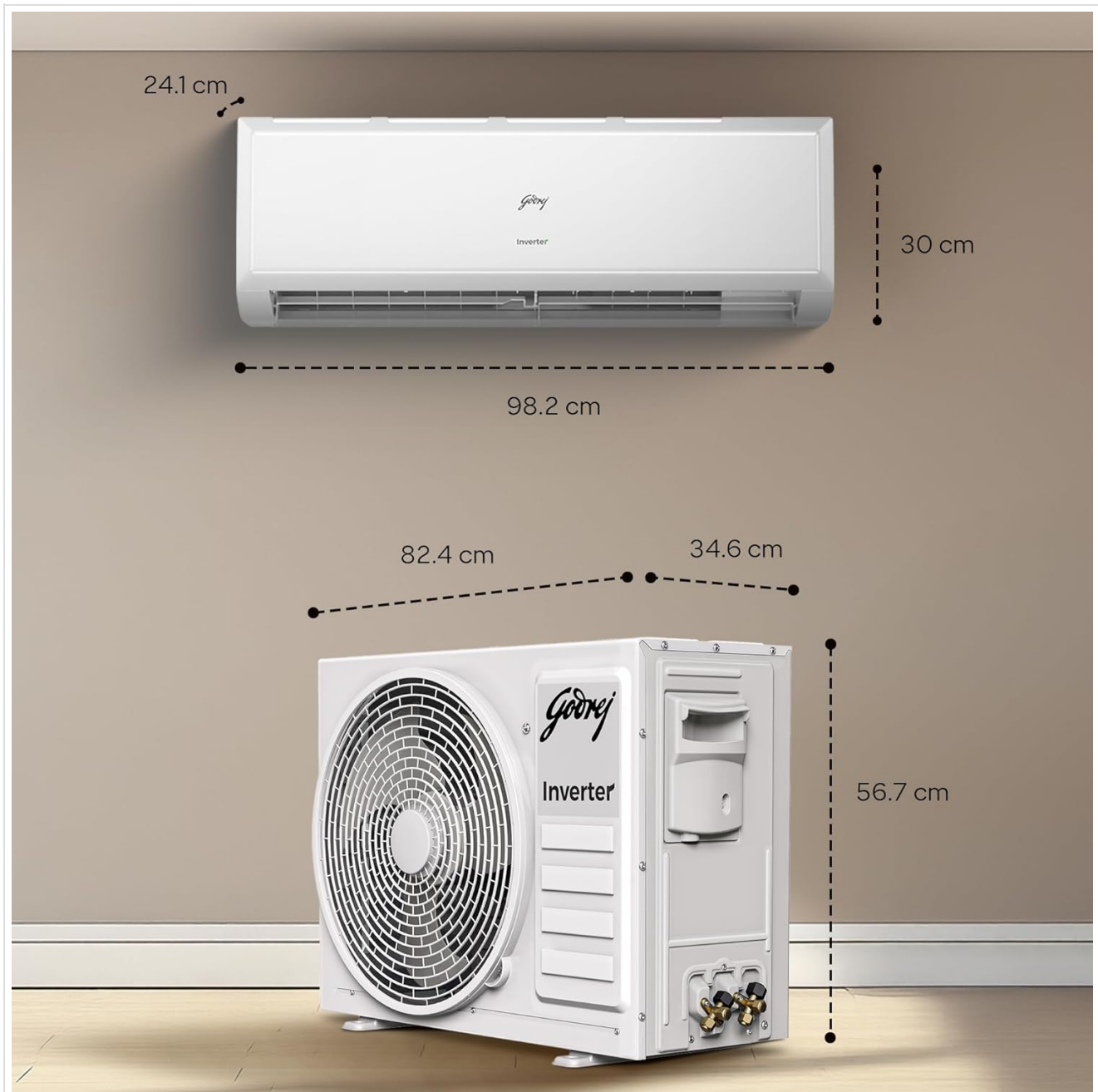
Image: A diagram illustrating the dimensions of both the indoor and outdoor units for proper installation planning.
